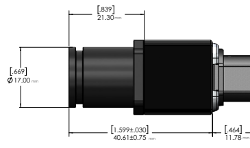
42° SIDE VIEW
