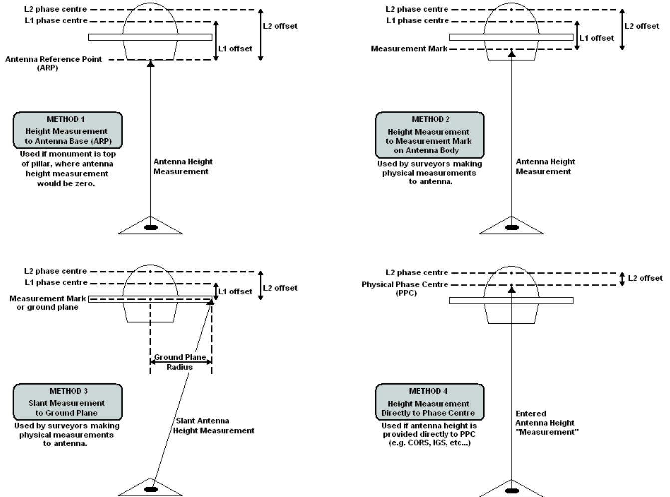
Figure 7: Antenna Measurements
